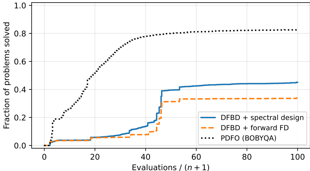
Data profile, \tau = 1e - 05 ( \sigma = 0.0001 )
