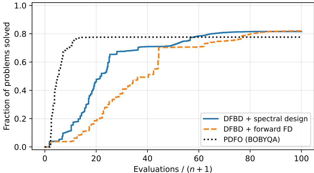
Data profile, \tau = 0.01 ( \sigma = 0.01 )
