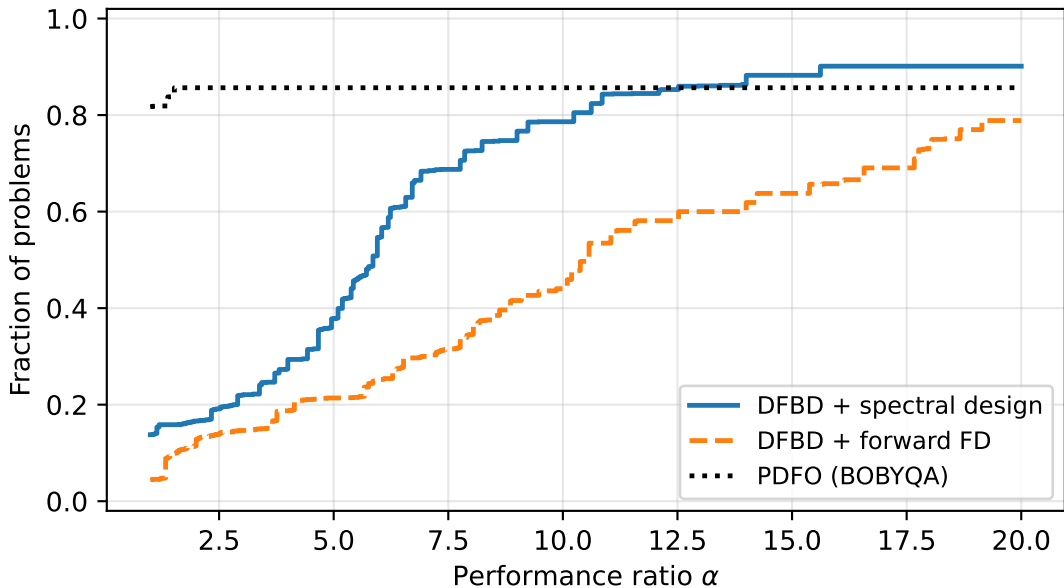
Performance profile, \tau = 0.1 ( \sigma = 0.01 )
