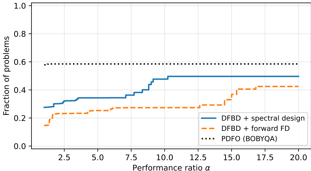
Performance profile, \tau = 1e - 05 ( \sigma = 0.01 )
