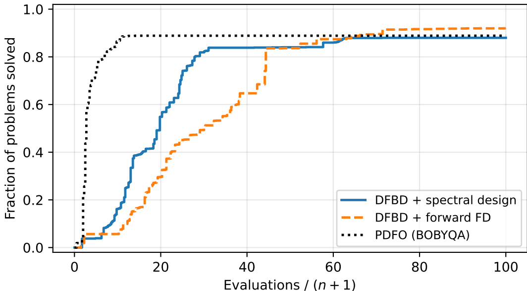
Data profile, \tau = 0.1 ( \sigma = 0.001 )
