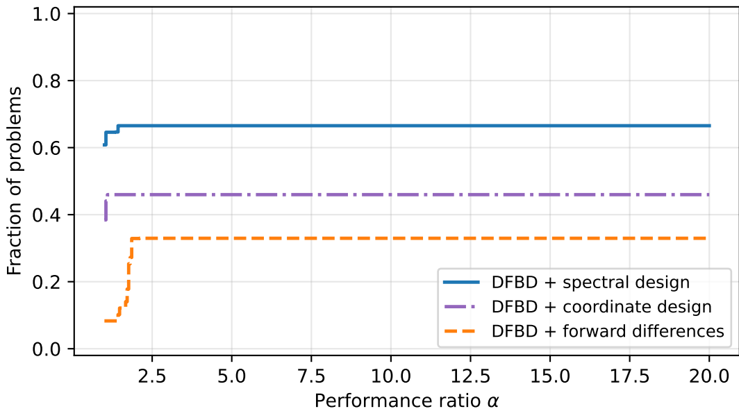
Performance profile, \tau = 1e - 07 ( \sigma = 0.01 )
