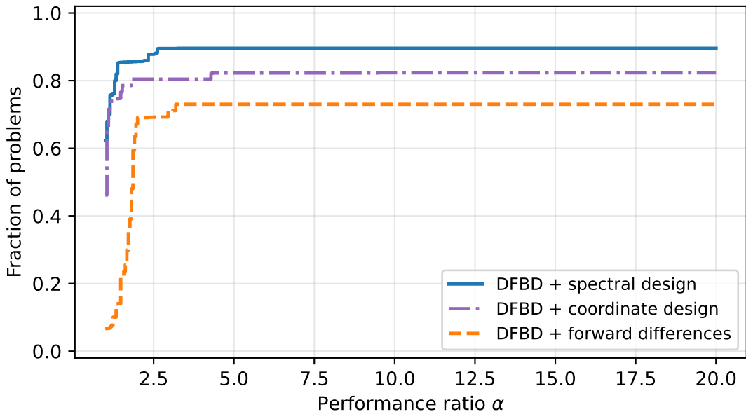
Performance profile, \tau = 0.01 ( \sigma = 0.001 )
