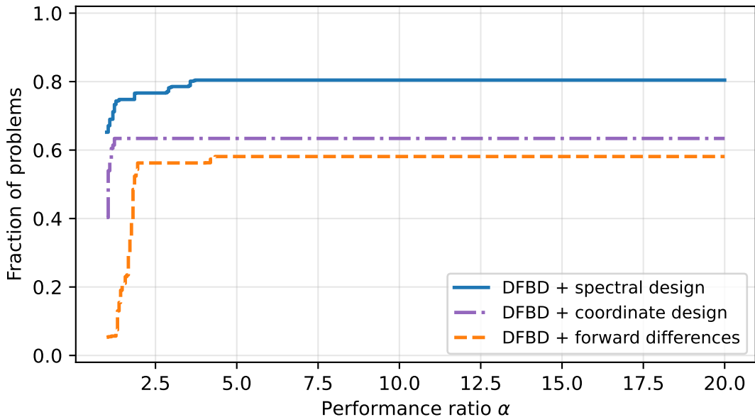
Performance profile, \tau = 0.001 ( \sigma = 0.001 )
