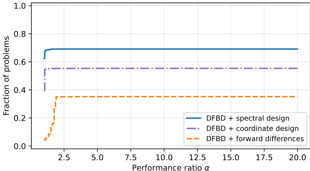
Performance profile, \tau = 1e - 05 ( \sigma = 0.0001 )
