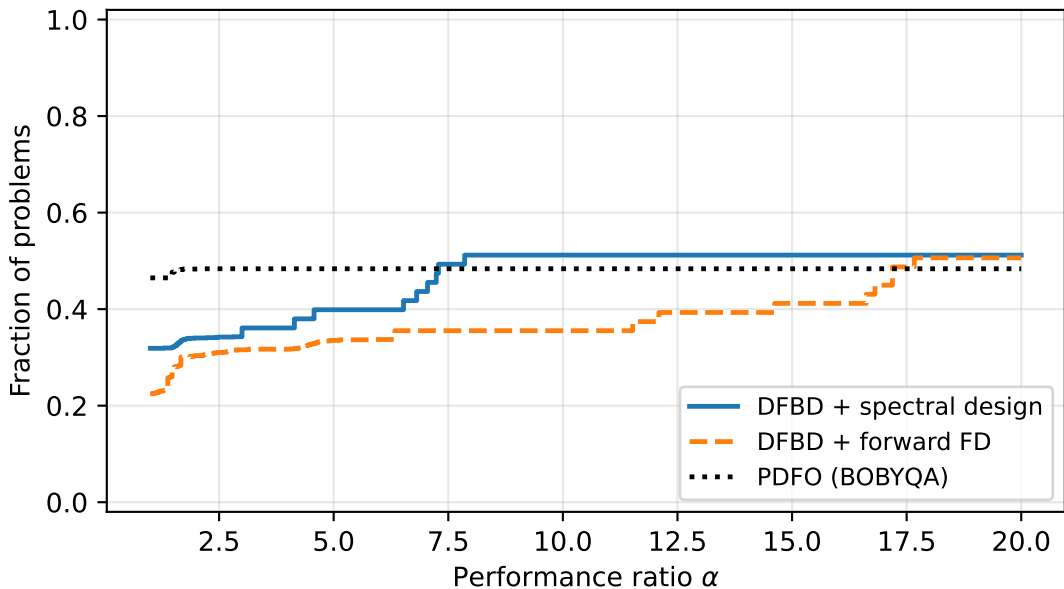
Performance profile, \tau = 1e-05 ( \sigma = 0.1 )
