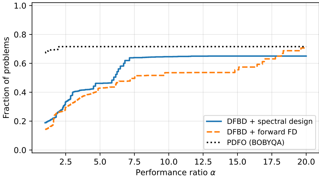
Performance profile, \tau = 0.001 ( \sigma = 0.01 )
