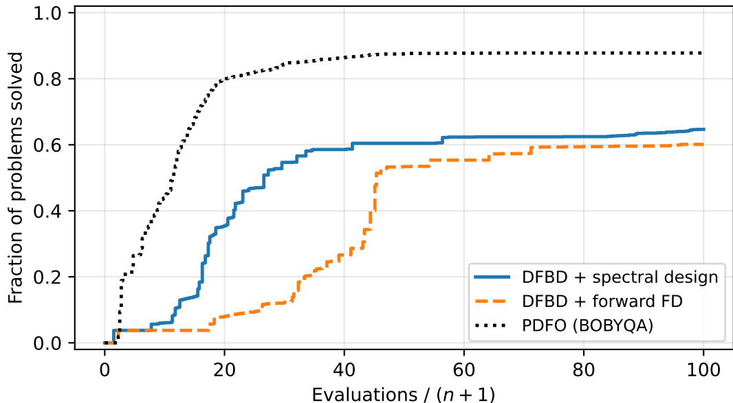
Data profile, \tau = 0.001 ( \sigma = 0.0001 )
