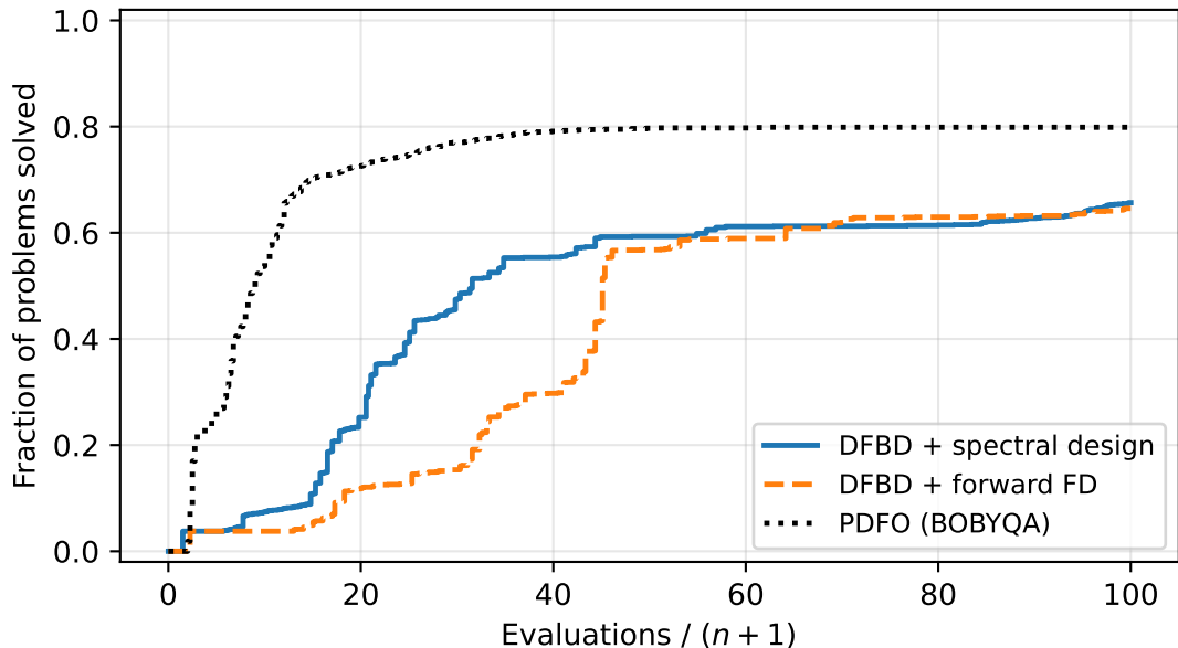
Data profile, \tau = 0.001 ( \sigma = 0.001 )
