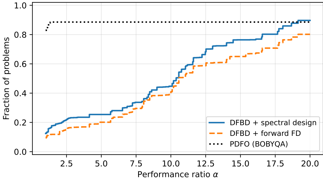
Performance profile, \tau = 0.1 ( \sigma = 0.001 )
