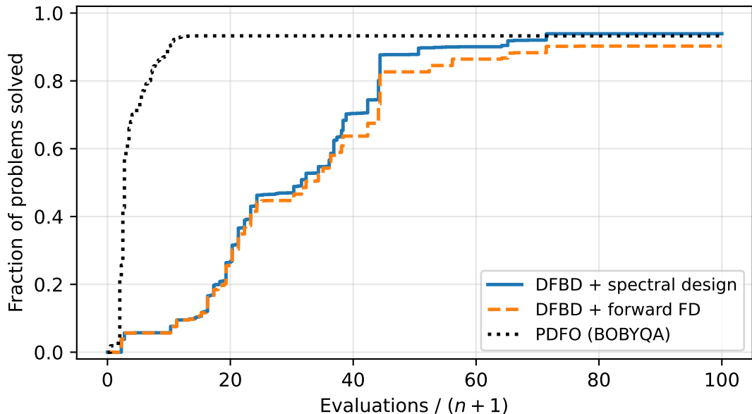
Data profile, \tau = 0.1 ( \sigma = 0.0001 )
