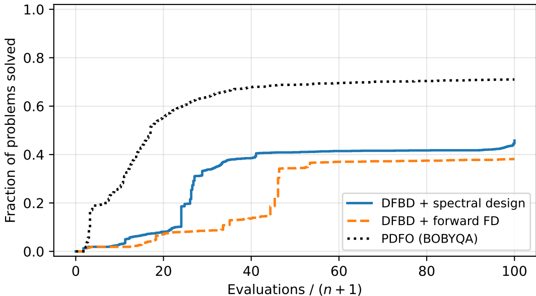
Data profile, \tau = 1e-05 ( \sigma = 0.001 )
