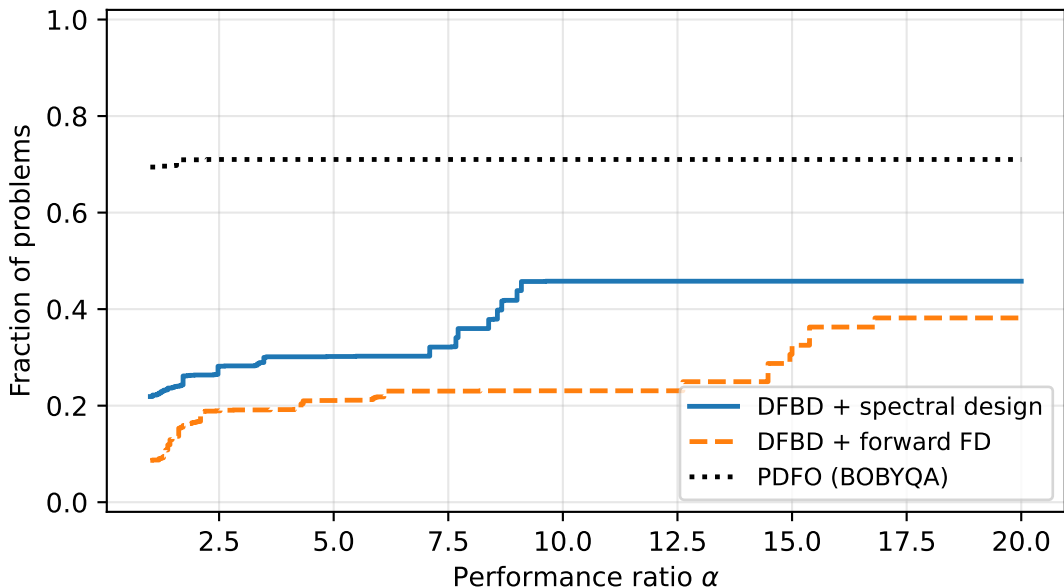
Performance profile, \tau = 1e - 05 ( \sigma = 0.001 )
