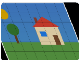
shear
