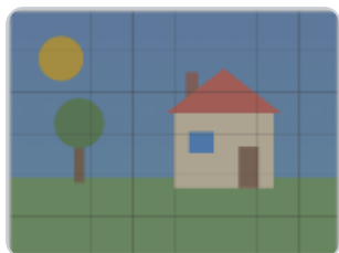
contrast -50%
