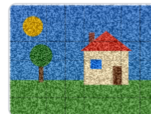
noise
