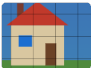
crop + resize
