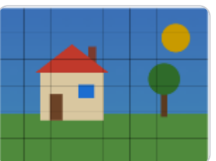
horizontal flip
