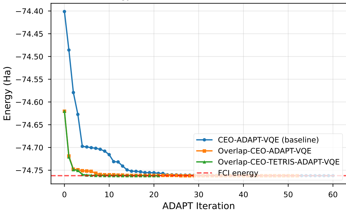
Absolute Energy — H 2 O STO-3G stretched (2.0 Å, frozen core)
