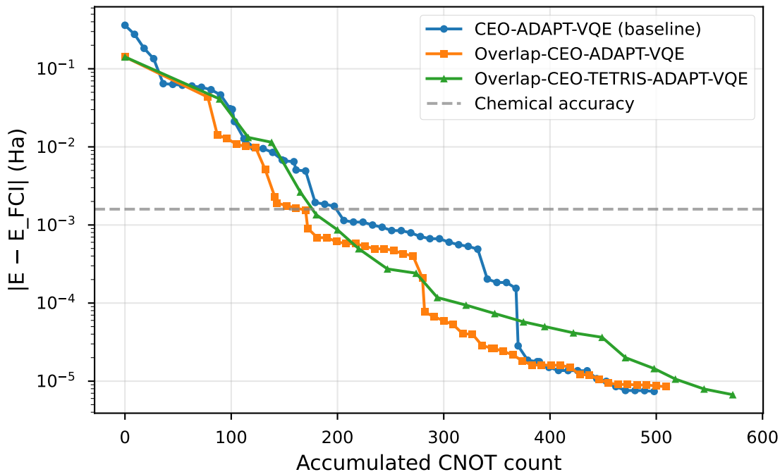
Energy vs CNOT Count — H 2 O STO-3G stretched (2.0 Å, frozen core)
