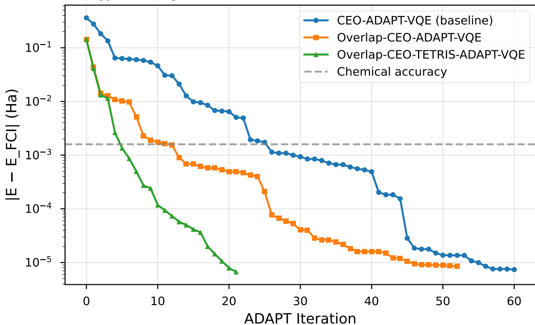
Energy Convergence — H 2 O STO-3G stretched (2.0 Å, frozen core)
