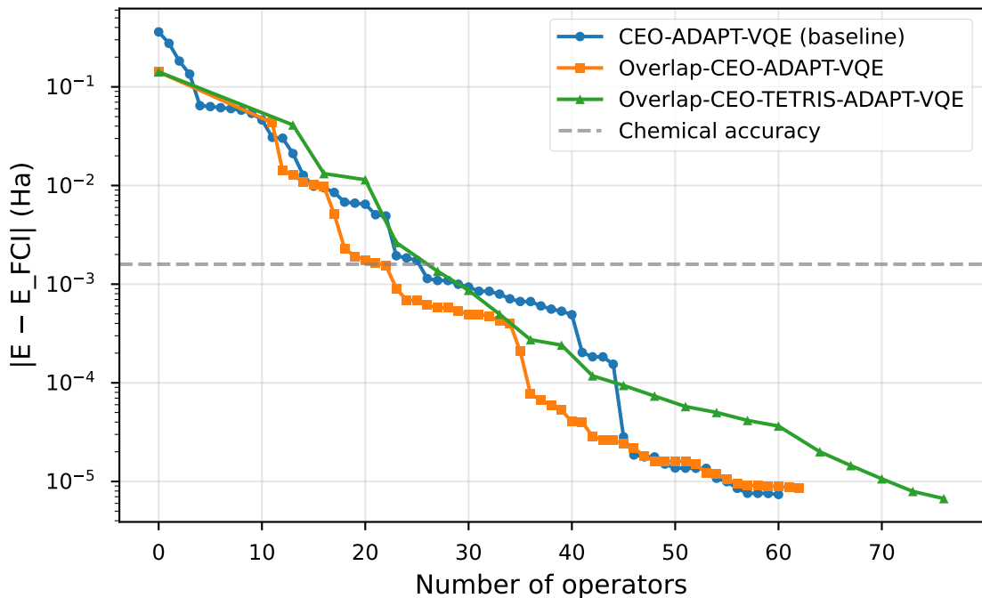
Energy vs Circuit Size — H 2 O STO-3G stretched (2.0 Å, frozen core)
