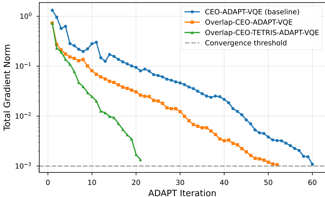
Gradient Norm — H 2 O STO-3G stretched (2.0 Å, frozen core)
