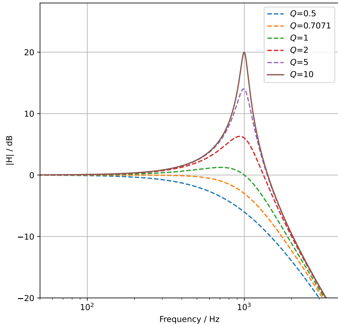
LPF Frequency Response for various Q ( H_0 = 1 )
