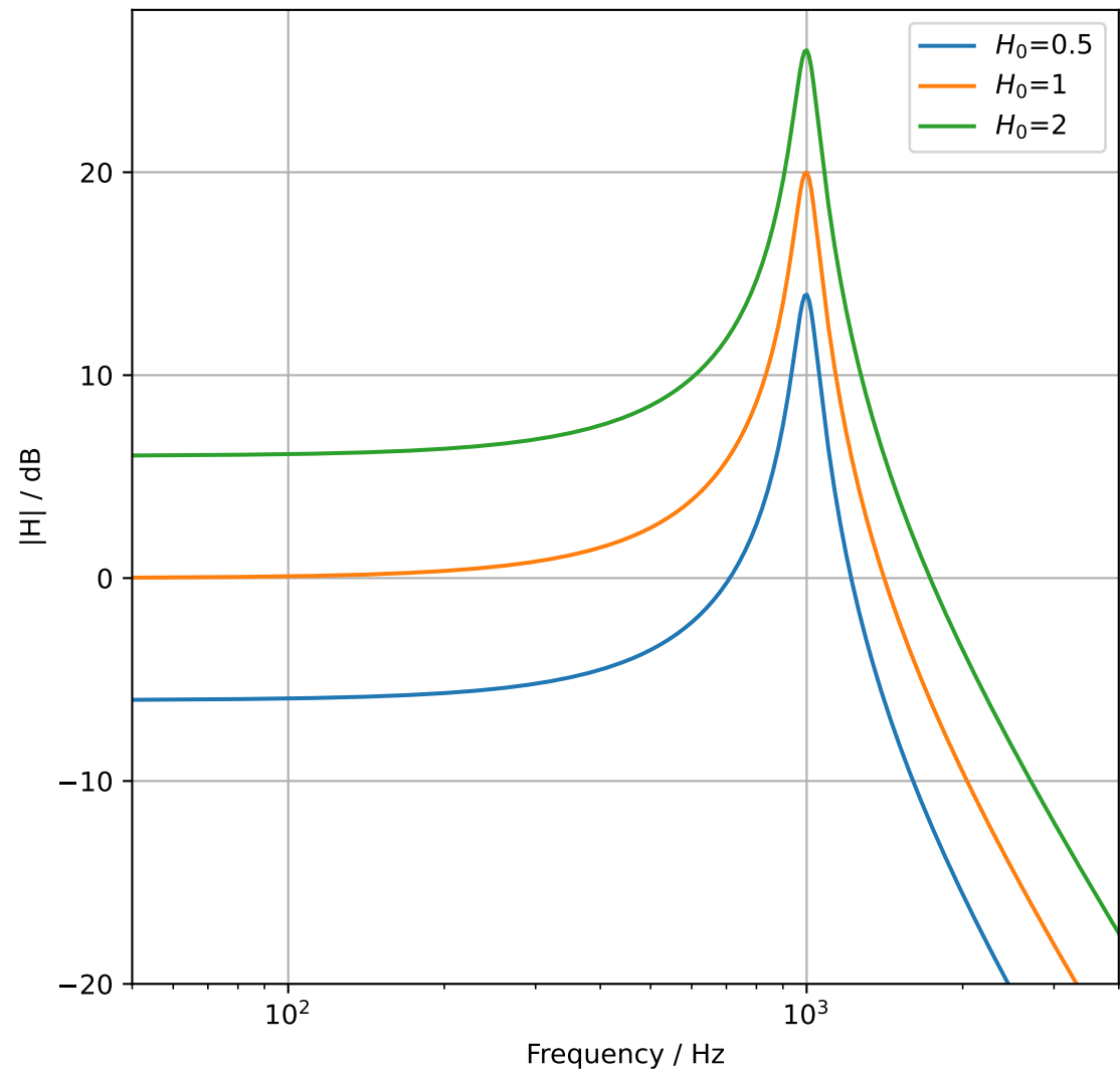
LPF Frequency Response for various H_0 ( Q = 10 )
