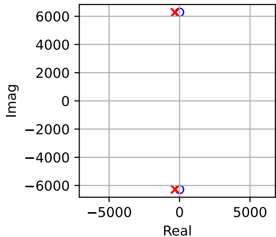
Bandstop Filter
