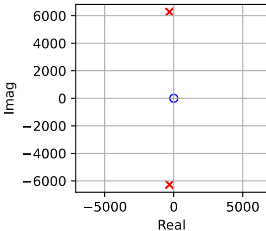
Bandpass Filter
