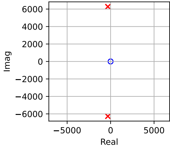
Highpass Filter
