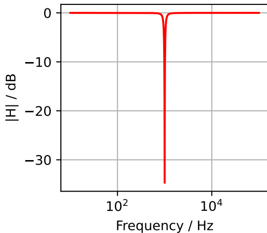
Bandstop Filter
