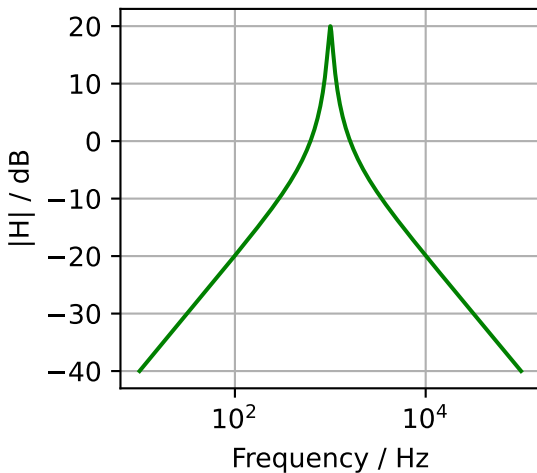
Bandpass Filter
