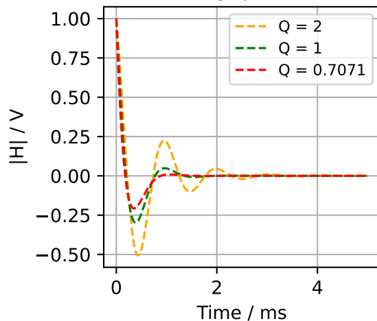
Highpass
