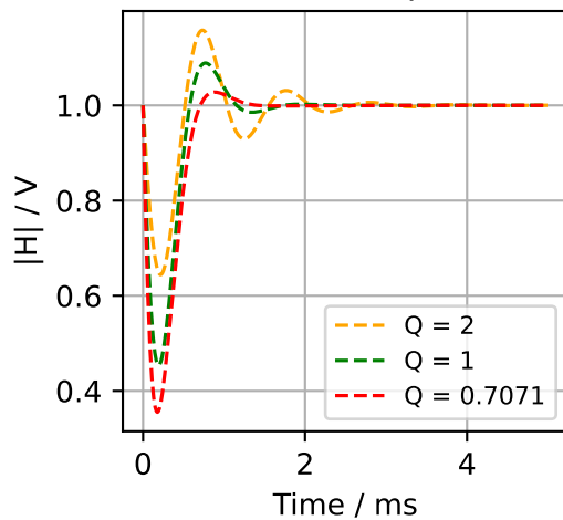
Bandstop
