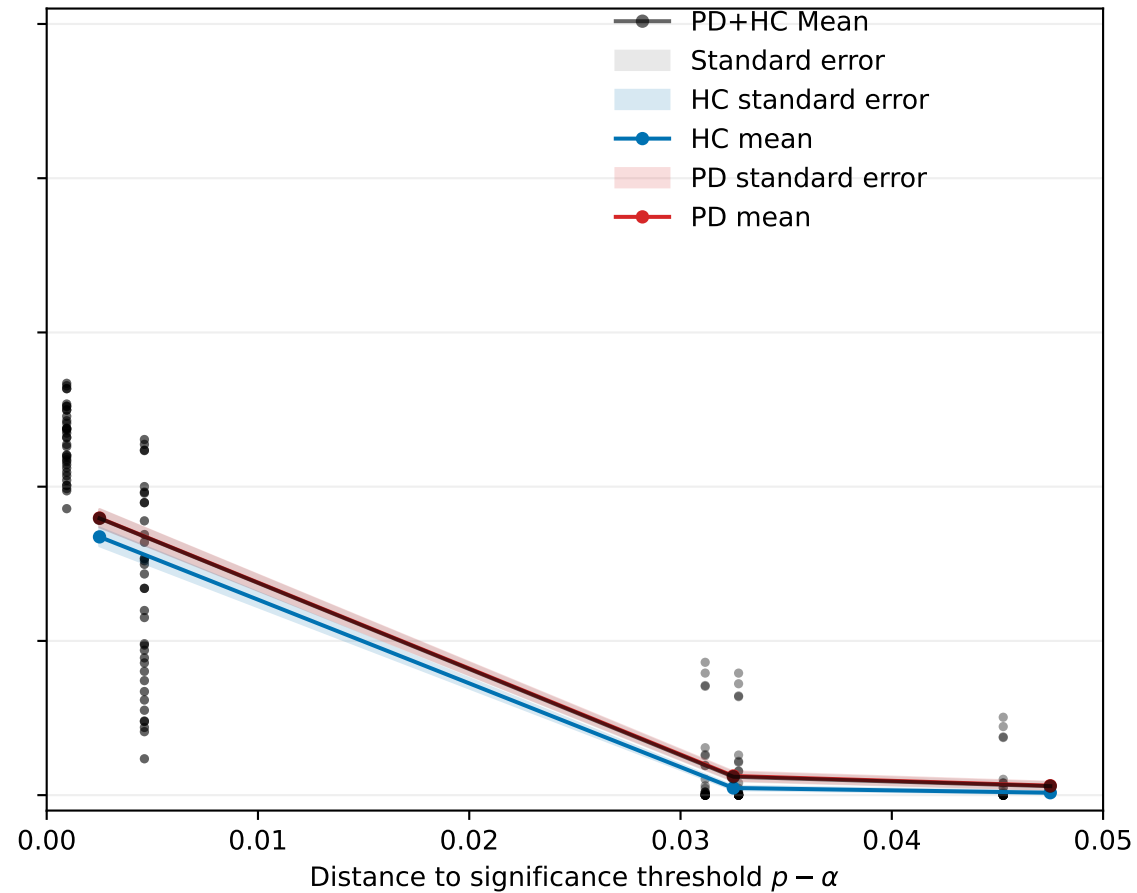
False-negative risk
