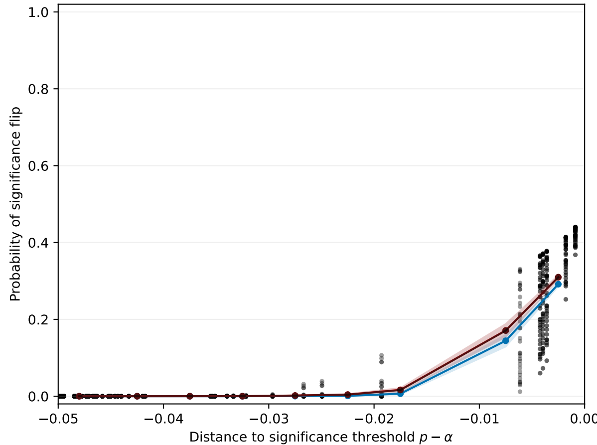
False-positive risk
