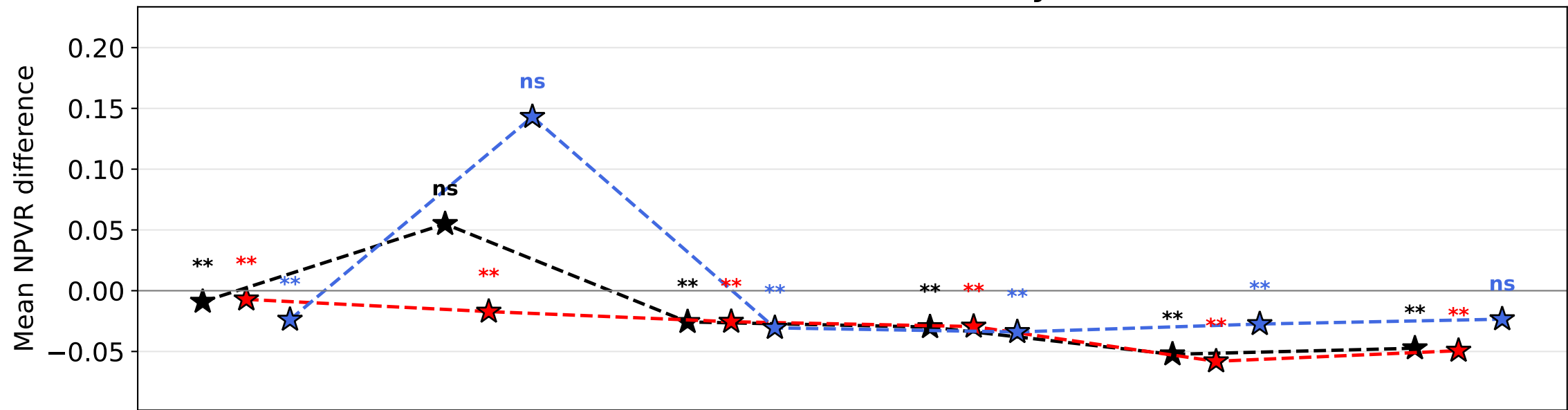
Eigenvector Centrality
