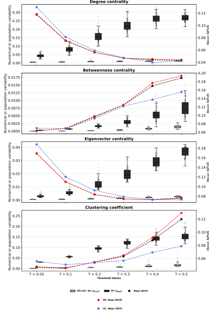
Figure 3.2: Numerical-to-population variability ratio for local graph metrics. Numerical variability (NV; \sigma_{\text{num}} ), population variability (PV; \sigma_{\text{pop}} ), and the mean numerical-to-population variability ratio (NPVR; \nu_{\text{npv}}^- ) across network thresholds. NPVR is shown for the pooled Parkinson’s disease (PD) and healthy control (HC) sample and separately for the PD and HC groups. Each point in a boxplot represents one brain region.
