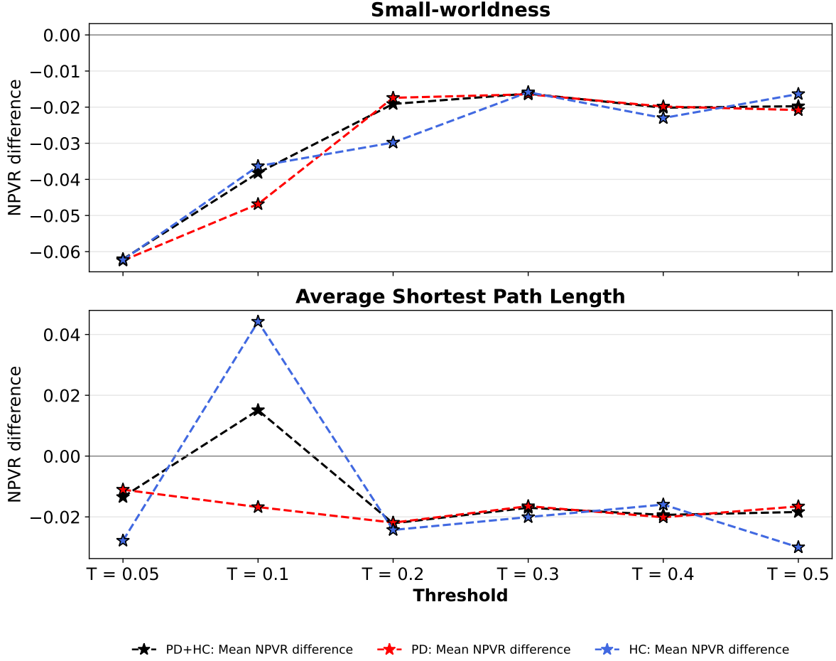
Figure 3.6: Numerical-to-population variability ratio differences across pipelines for global graph metrics. Numerical-to-population variability ratio (NPVR) differences between the no-confound and with-confound pipelines, calculated as no-confound minus with-confound , for small-worldness and average shortest path length across network thresholds. Results are shown for the pooled Parkinson’s disease (PD) and healthy control (HC) sample (black), PD group (red), and HC group (blue). All populations were evaluated using the same network thresholds: T = 0.05, 0.10, 0.20, 0.30, 0.40 , and 0.50 . Markers were shifted slightly along the horizontal axis to prevent overlap and improve visualization; these offsets do not represent different threshold values.
