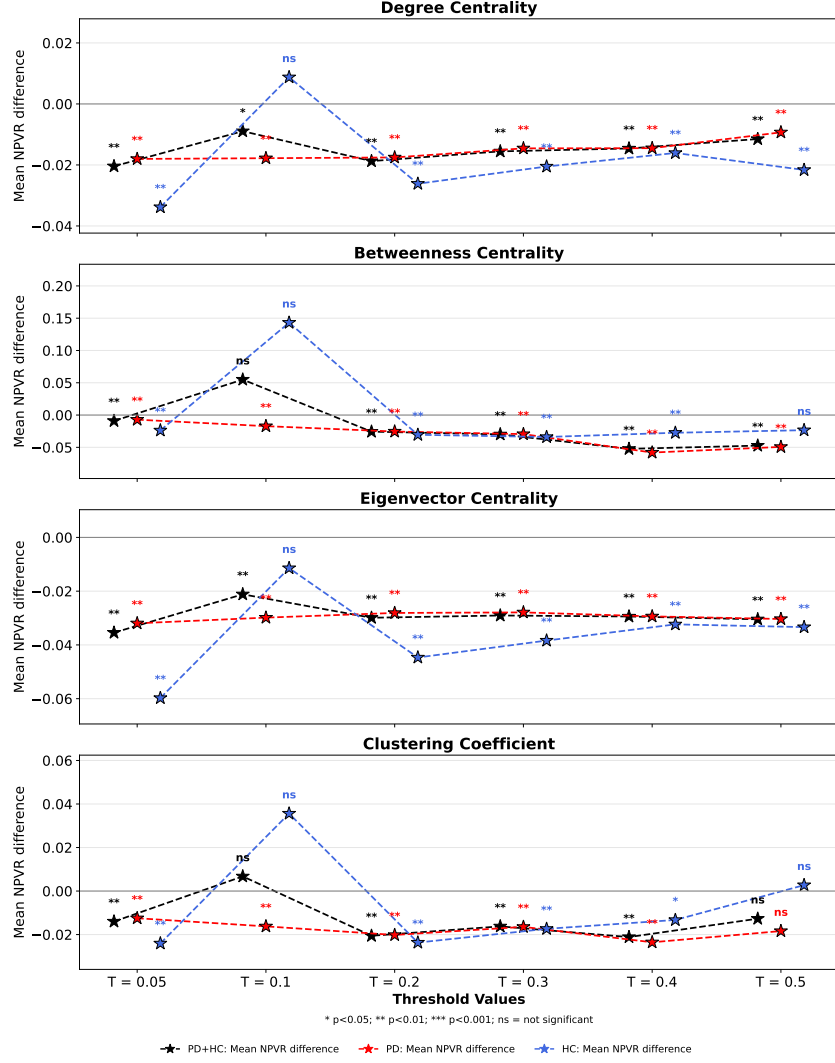
Figure 3.5: Numerical-to-population variability ratio differences across pipelines for local graph metrics. Region-averaged numerical-to-population variability ratio (NPVR) differences between the no-confound and with-confound pipelines, calculated as no-confound minus with-confound . Results are shown for the pooled Parkinson’s disease (PD) and healthy control (HC) sample (black), PD group (red), and HC group (blue). All populations were evaluated using the same network thresholds: T = 0.05, 0.10, 0.20, 0.30, 0.40 , and 0.50 . Markers were shifted slightly along the horizontal axis to prevent overlap and improve visualization; these offsets do not represent different threshold values.
