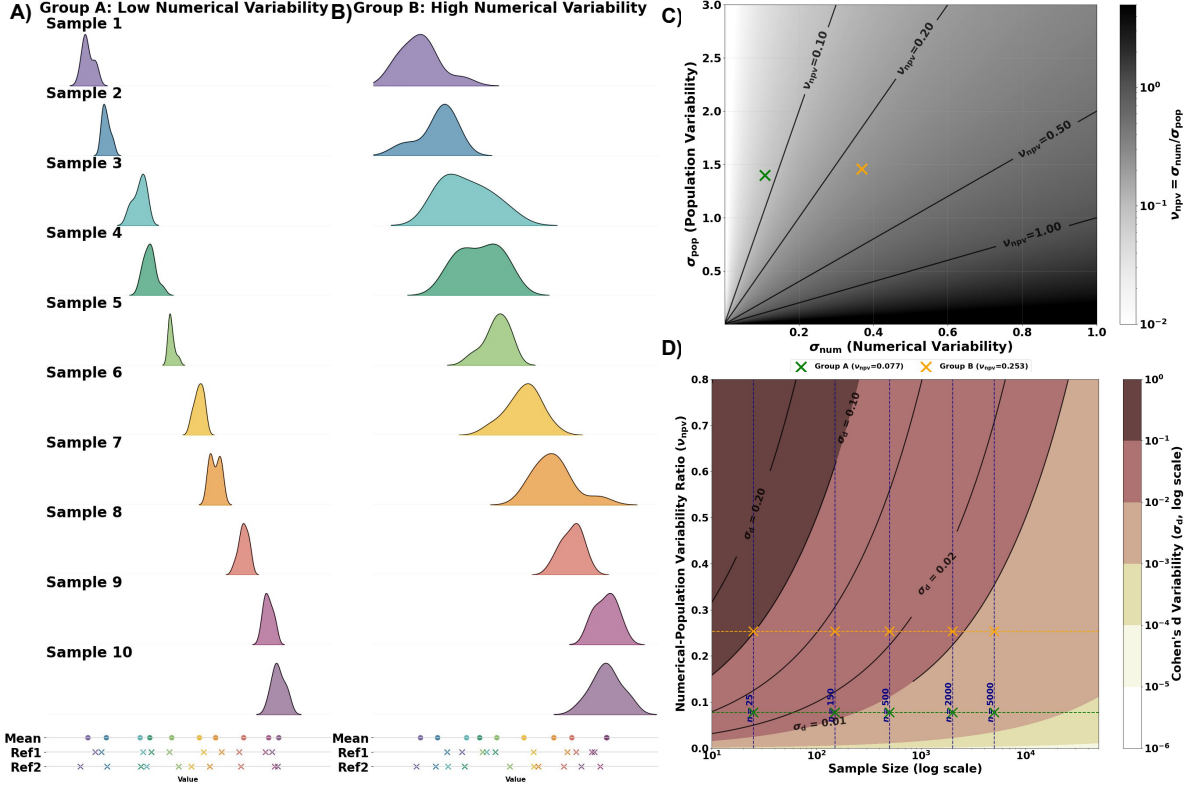
Figure 3.1: Impact of numerical variability on inference. (A–B) Simulated distributions of measurement values from two populations (10 subjects each) under low (A) and high (B) within-individual numerical variability. (C) Numerical-to-population variability ratio (NPVR; \nu_{npvr} ) computed for the two populations. (D) Propagated numerical standard deviation of Cohen's d , \sigma_d = 2\nu_{npvr}/\sqrt{n} , as a function of sample size and NPVR. Darker shading indicates greater numerical uncertainty in Cohen's d , and lighter shading indicates lower uncertainty. Vertical dashed lines indicate selected example sample sizes.
