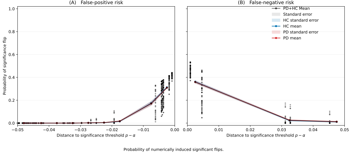
Figure 3.7: Probability of numerically induced significance flips. Significance-flip probability as a function of the distance between the nominal p -value and the significance threshold, p_0 - \alpha , with \alpha = 0.05 . Individual points represent configurations from the pooled Parkinson’s disease and healthy control (PD+HC) analysis across graph metrics, network thresholds, sample sizes, representative test-statistic values, and statistical tests. The left panel (A) shows nominally significant results that may become non-significant, whereas the right panel (B) shows nominally non-significant results that may become significant. Lines represent mean flip probabilities calculated in bins of width 0.005 for the pooled PD+HC sample (black), Parkinson’s disease (PD) group (red), and healthy control (HC) group (blue). Shaded regions represent the corresponding standard errors. The false-positive and false-negative labels describe instability of the nominal significance classification rather than classical error rates based on known ground truth.
