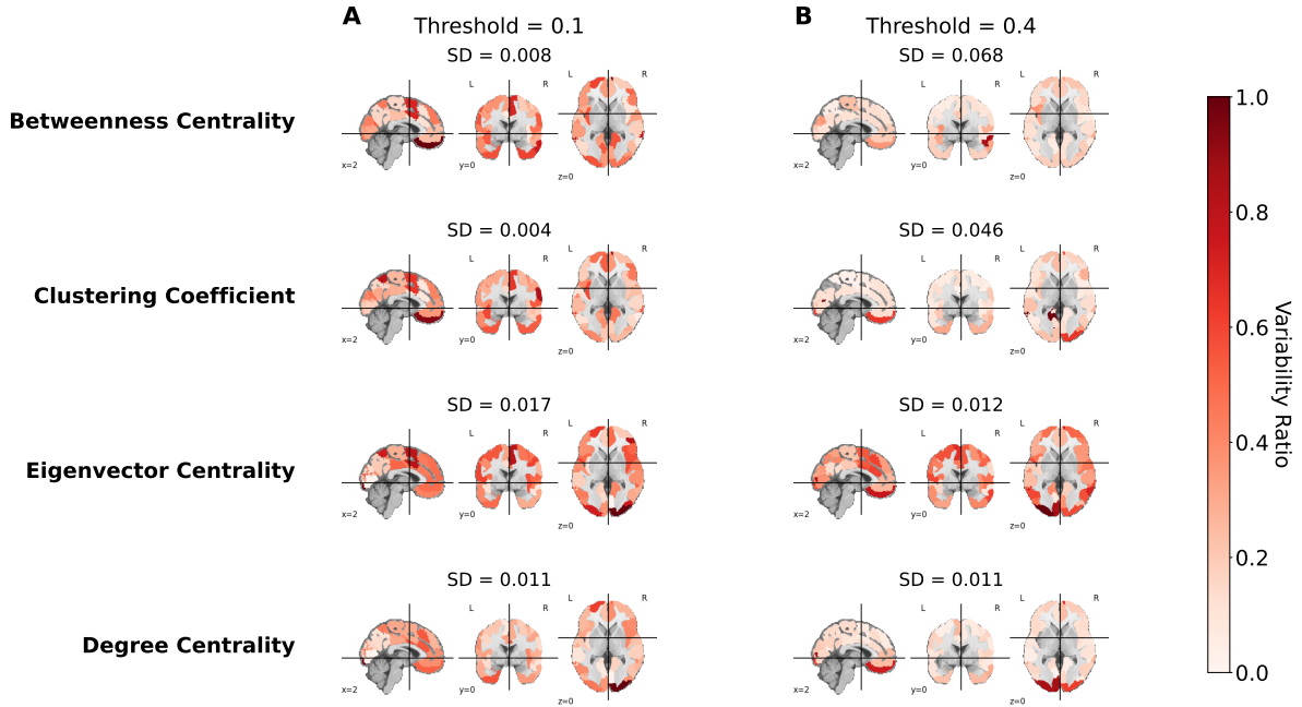
Figure 3.4: Numerical-to-population variability ratio across brain regions. Normalized regional numerical-to-population variability ratio (NPVR) maps for the pooled Parkinson’s disease (PD) and healthy control (HC) sample at (A) threshold 0.1 and (B) threshold 0.4. Rows show betweenness centrality, clustering coefficient, eigenvector centrality, and degree centrality. Values are normalized independently within each metric and threshold, with darker red indicating a higher NPVR. SD denotes the regional standard deviation of the NPVR.
