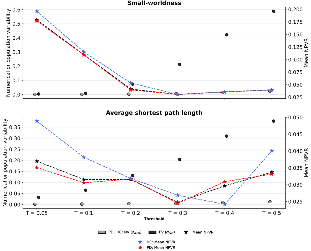
Figure 3.3: Numerical-to-population variability ratio for global graph metrics. Numerical variability (NV; \sigma_{num} ), population variability (PV; \sigma_{pop} ), and the mean numerical-to-population variability ratio (NPVR; \nu_{npv}^- ) across network thresholds. NPVR is shown for the pooled Parkinson’s disease (PD) and healthy control (HC) sample and separately for the PD and HC groups.
