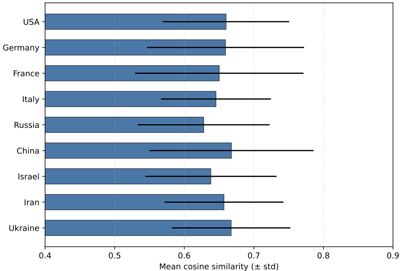
LLaMA 3.1-70B: Role-based vs. Assistant similarities
