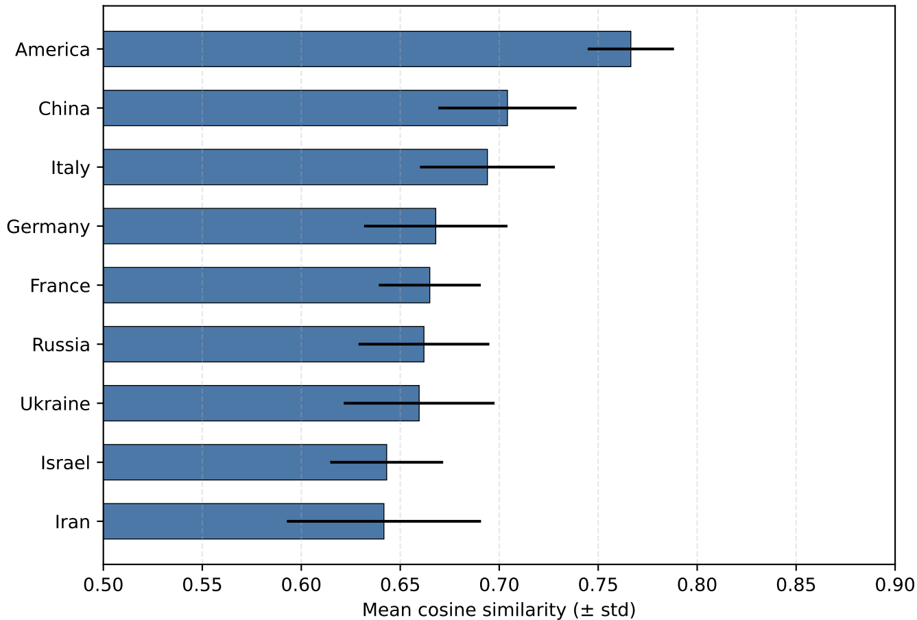
GPT-4o-mini: Role-based vs. Native similarities
