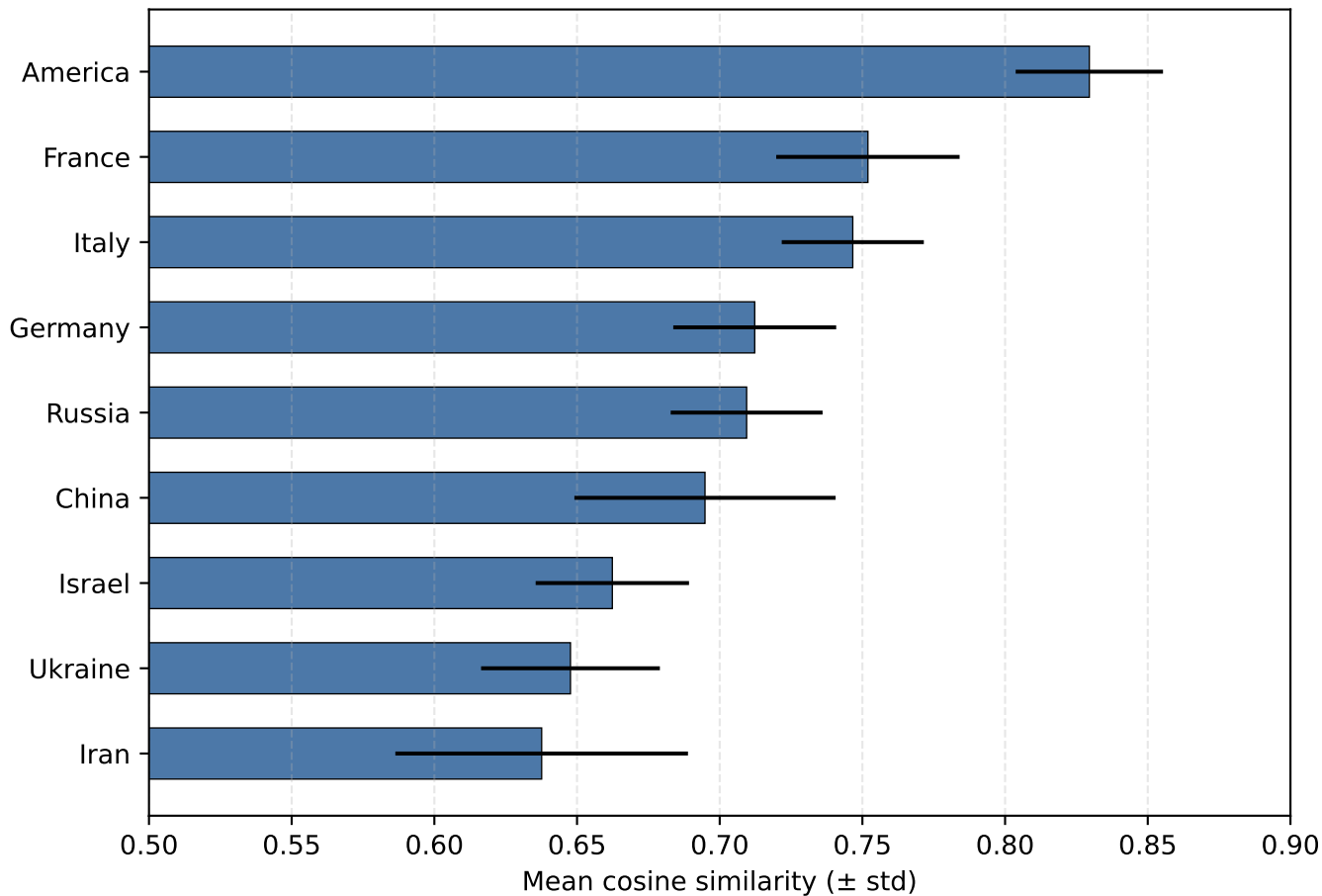
LLaMA 3.1-70B: Native vs. Role-based similarities
