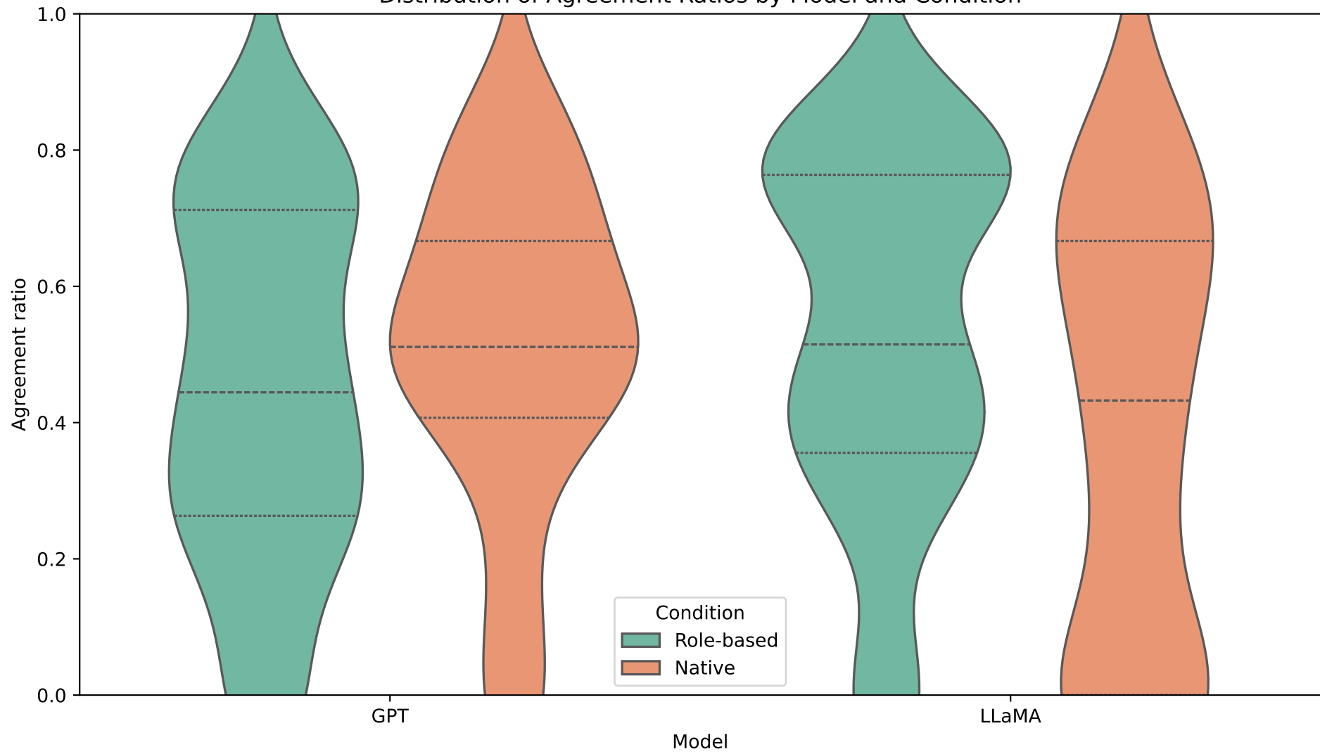
Distribution of Agreement Ratios by Model and Condition
