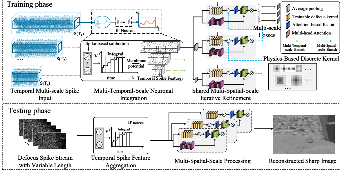
Figure 4. Overview of the proposed DeSpoke framework. The framework consists of two phases. During training, temporally multi-scale spike streams are integrated using a bank of integrate-and-fire (IF) neurons to capture spike dynamics at temporal scales. These features are fed into a shared multi-spatial-scale iterative refinement module, guided by physics-based discrete PSF priors. Transformer-based attention is used to fuse features across both temporal and spatial scales. Multi-scale losses are applied at each refinement level to supervise reconstruction. During inference, a defocus spike stream with variable length is temporally aggregated and passed through the learned spatial-scale fusion module to produce a sharp intensity reconstruction.
