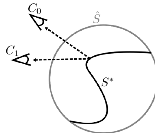
Shape-Radiance Ambiguity
