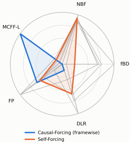
I2V @ 60 s
