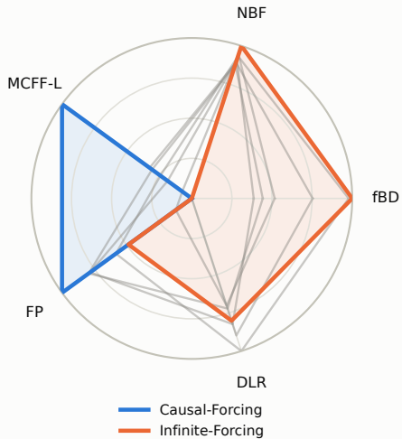
T2V @ 60 s
