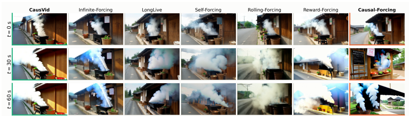
Figure 3. Every audited system on one prompt. Columns are ordered by increasing static-region drift. The two highlighted systems are the pair a whole-frame motion score cannot separate: the leftmost holds its support fixed while its smoke continues to rise, the rightmost has relocated the scene entirely by t = 30 s.
