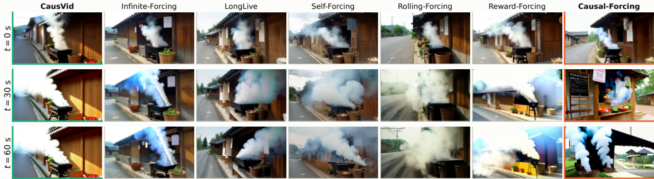
One prompt, every audited system, ordered left-to-right by increasing static-region drift (fBD). Released 60 s generations; the two highlighted systems are the pair a whole-frame motion score cannot separate.
