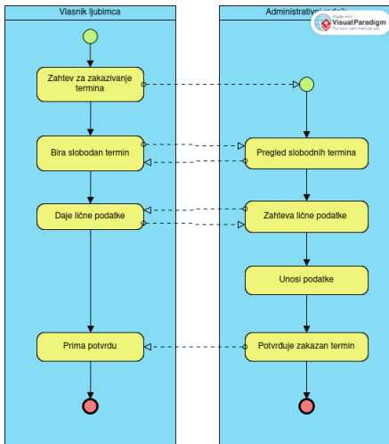
Figure: BPMN diagram
