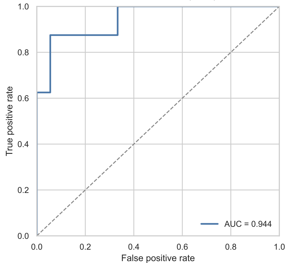
B. PCG ROC curve (n=26)
