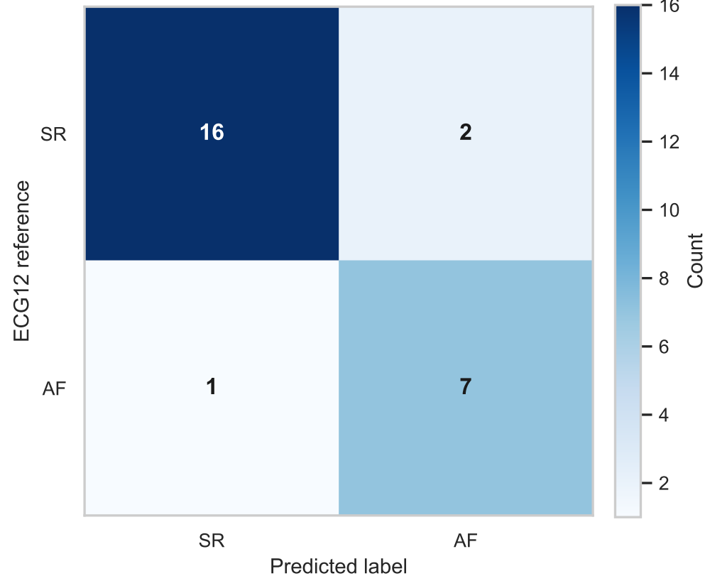
A. Confusion matrix (n=26 decided)
