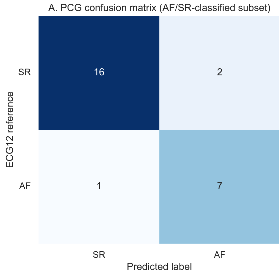
Figure 3. PCG decided-subset performance
