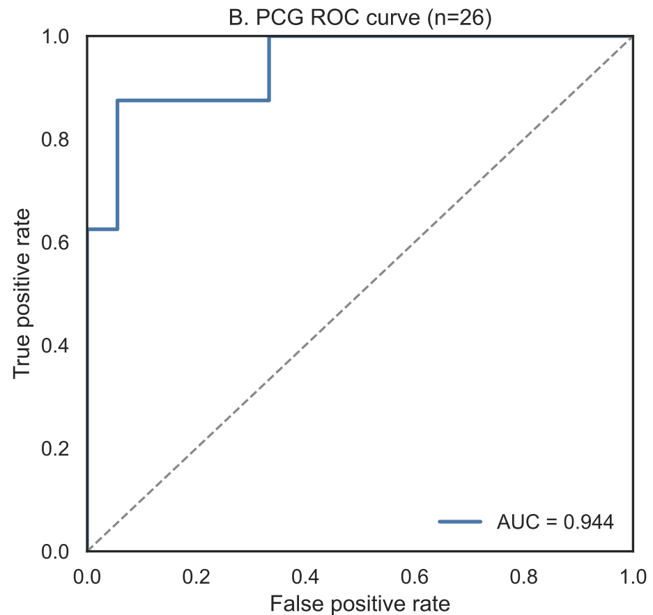
Figure 3. PCG decided-subset performance
