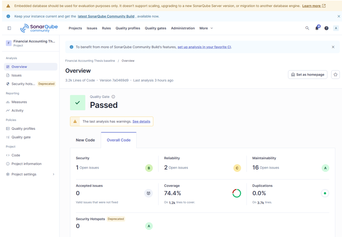
Figure F.1. SonarQube baseline overview dashboard.
