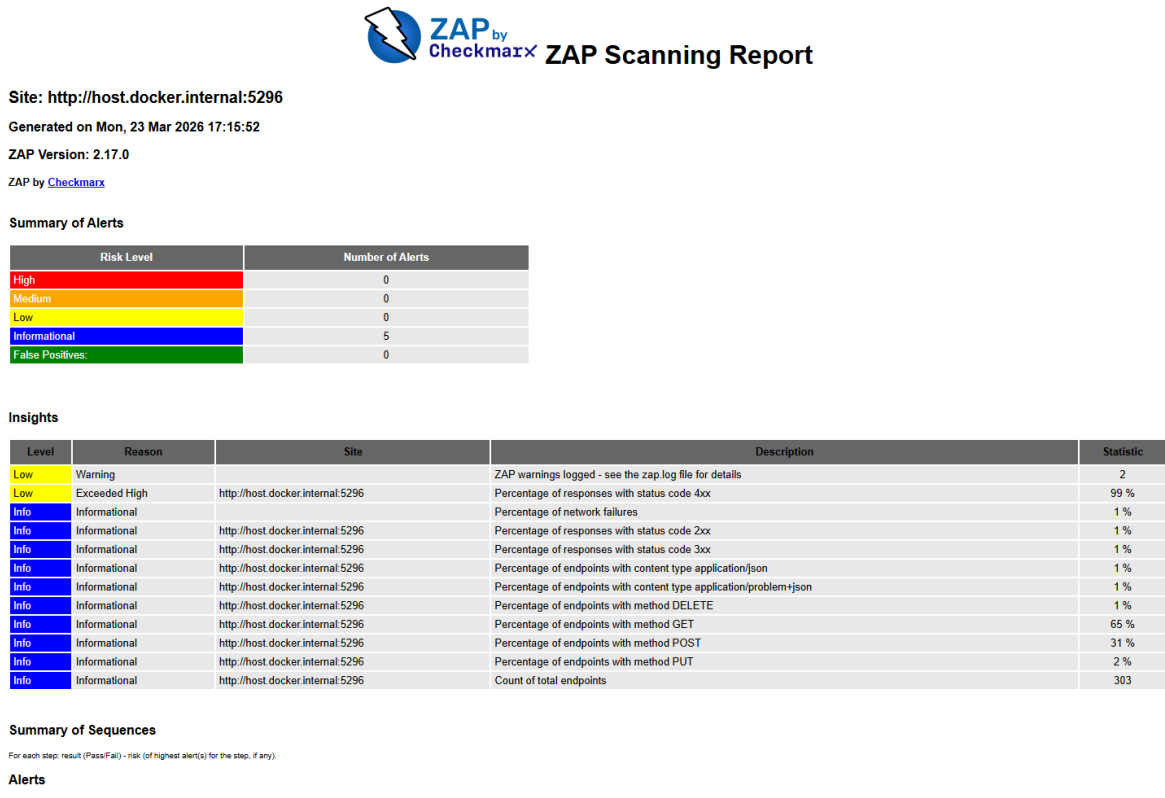
Figure F.8. OWASP ZAP api after summary dashboard.
