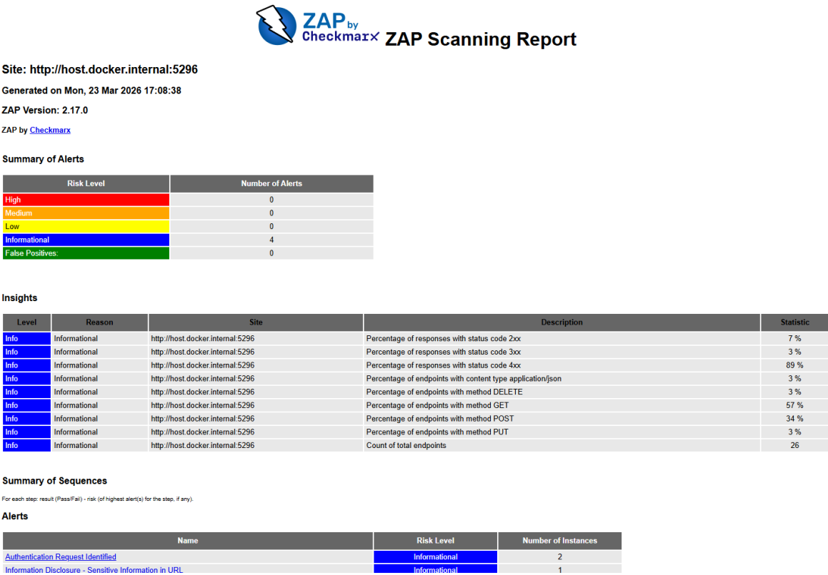
Figure F.6. OWASP ZAP baseline after summary dashboard.
