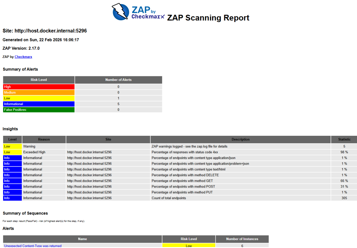
Figure F.7. OWASP ZAP api before summary dashboard.
