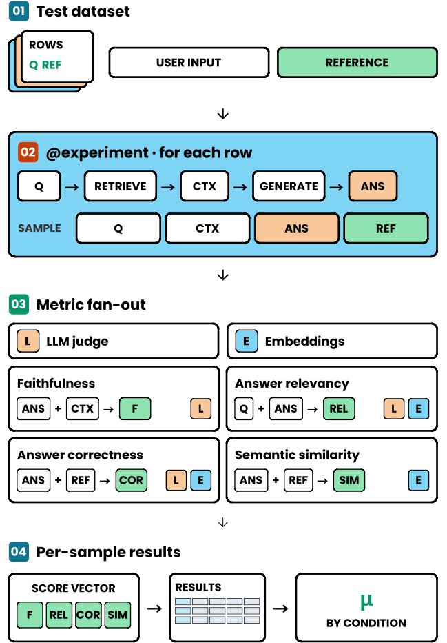
Fig. 3. RAGAS response-evaluation workflow from per-question inputs and evidence to per-condition results.
