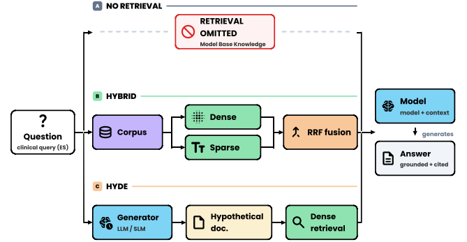
Fig. 2. RAG variants used in the benchmark: No RAG, Hybrid retrieval with dense and sparse fusion, and independent HyDE retrieval.
