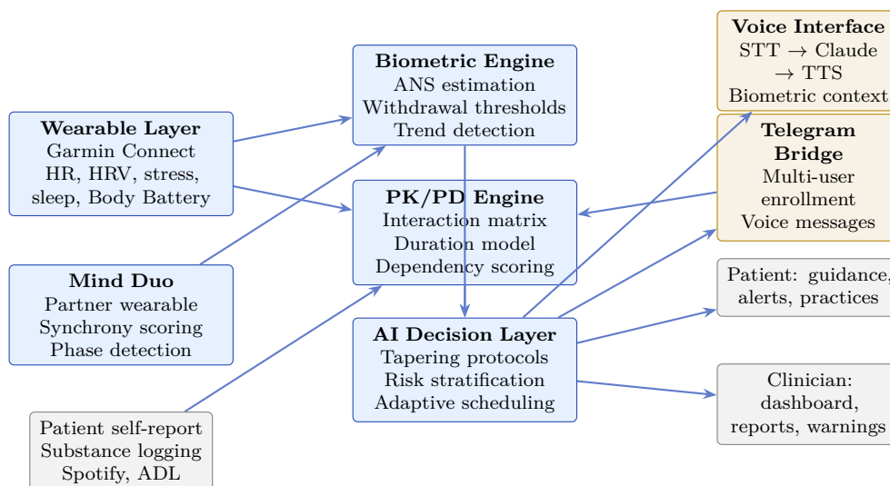
Figure 2: Mind Protocol system architecture. Orange boxes indicate patient-facing interfaces; blue boxes indicate processing layers. Arrows show data flow.
