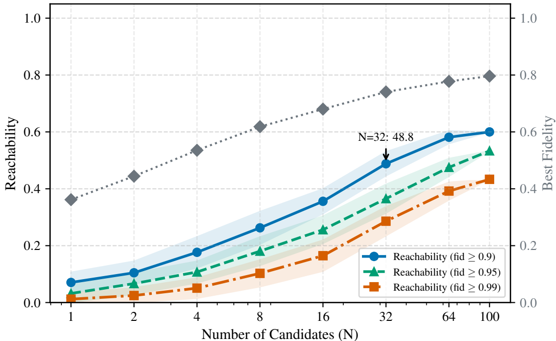
Best-of-N: Reachability vs Candidate Count
