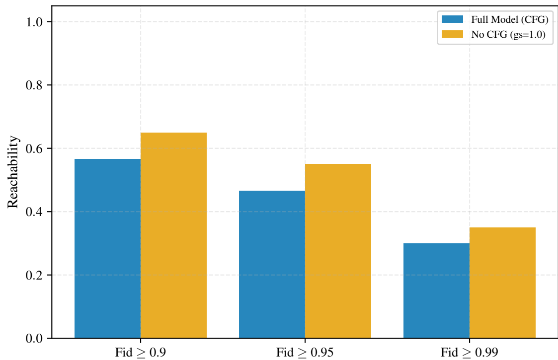
CFG Ablation
