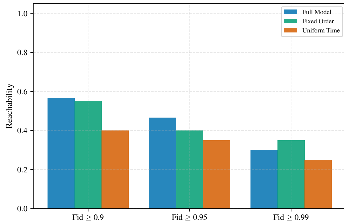
Branch Ablation
